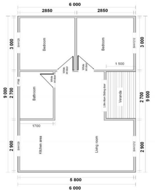
6x9m TWO BEDROOM
