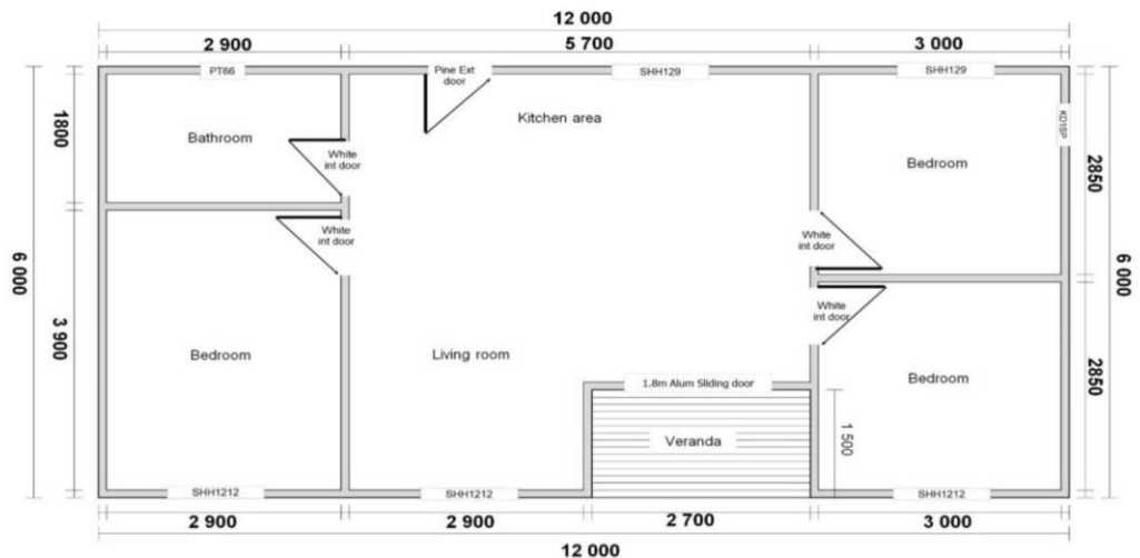
6x12m THREE BEDROOM
